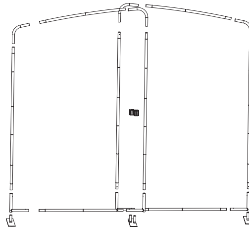
Assembly Plan
