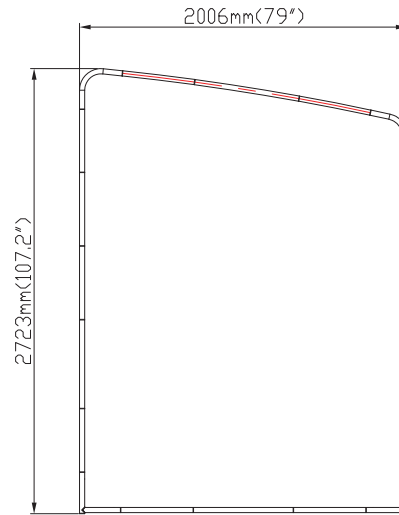
Media Frame w79xh107.2" WL-2000C
